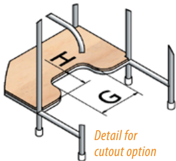
Extended intermediate rails with cutout option
